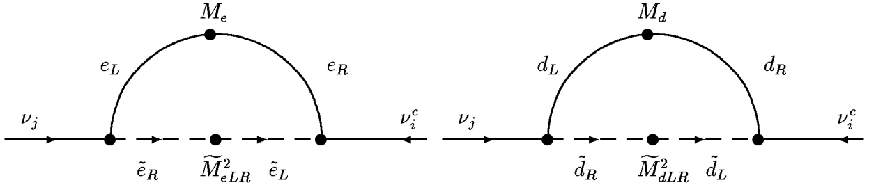
FIG. 1. Radiative generation of neutrino Majorana mass
