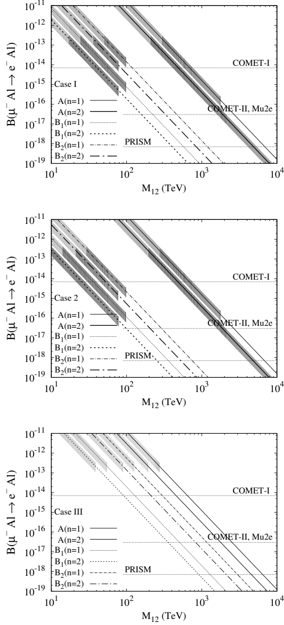
Figure 1: M_{12} dependence of B(\mu^- \text{Al} \rightarrow e^- \text{Al}) for U_u = \mathbf{1} and U_d = V_{\text{CKM}} (upper panel), for U_u = V_{\text{CKM}}^\dagger and U_d = \mathbf{1} (middle panel), and for U^u = \tilde{U}^u and U^d = \tilde{U}^d (see Eq. (2.18)) (lower panel). Light and dark shaded region is excluded region by the SINDRUM-II and by the observed P^0 - \bar{P}^0 mixing (Table 1), respectively. Horizontal dashed lines show the single event sensitivities of each experiment (see Introduction).
